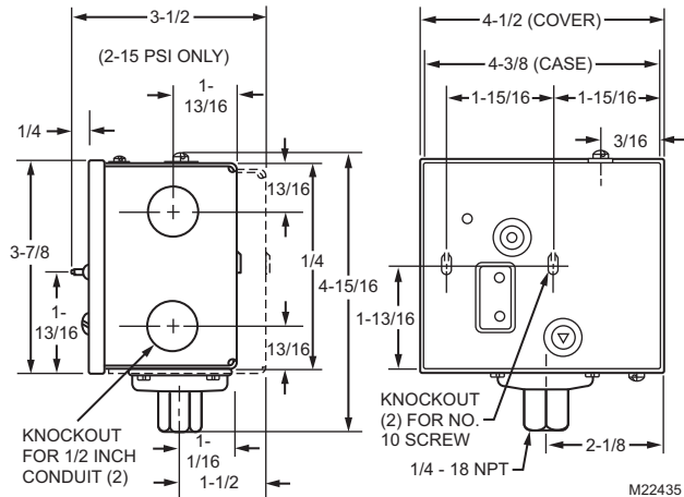
Fig. 1. L4079A,B,W PressureTrol® Limit Control dimensions in inches.
